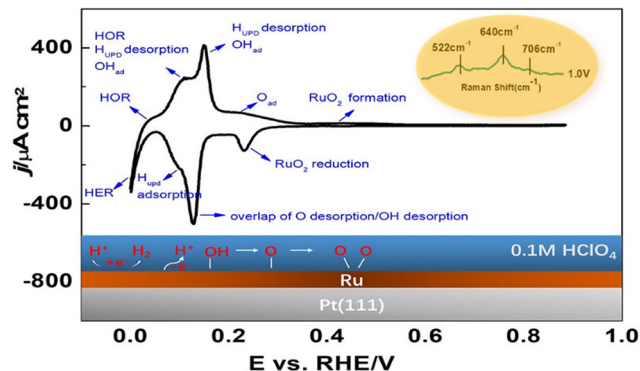
Fig. 9 Depicted surface processes on Ru/Pt(111) in 0.1 M HClO 4 . 193 Reprinted with permission from ref. 193. Copyright 2022 American Chemical Society.
