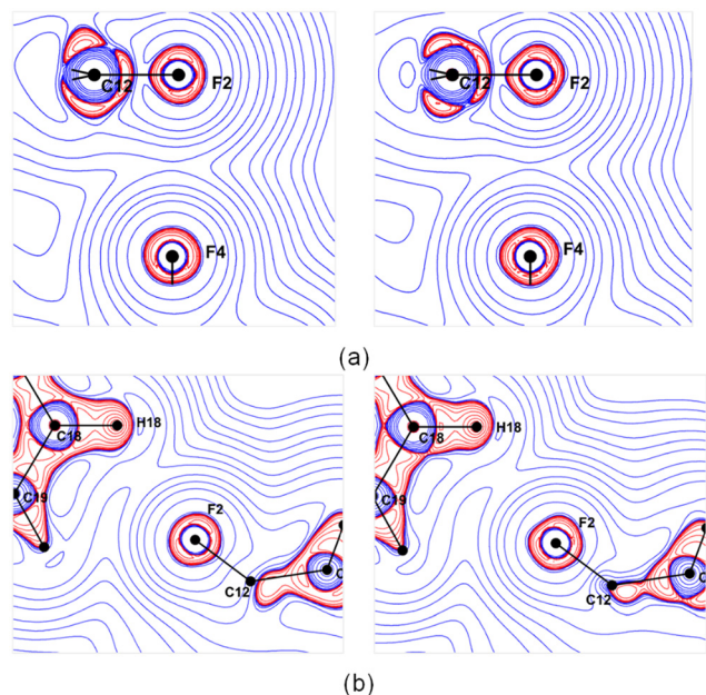
Fig. 7 Experimental (left) and theoretical (right) Laplacian maps for (a) C12-F2...F4-C10 interaction and (b) C18-H18...F2-C12 hydrogen bond drawn at the logarithmic interval of -\nabla^2\rho e Å -3 .
