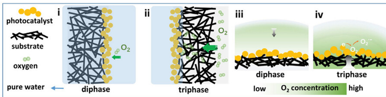
Fig. 14 Schematic illustration of diphase and triphase photocatalytic conditions. Adapted with permission from ref. 146. Copyright 2021 Wiley.
