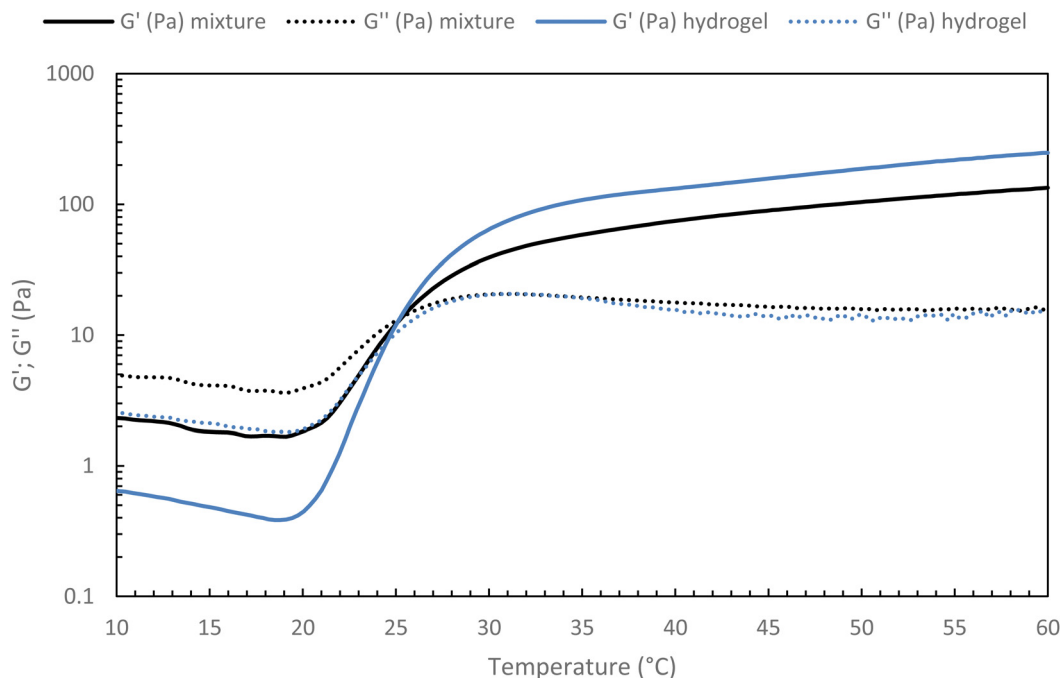
Fig. 10 Temperature ramp for hydrogel alone (HA- g -P(iPrOx-co-PBuOx-67/33)-0.10) and hydrogel/HA mixture (75/25 – v/v) at 15 \text{ g L}^{-1} in NaCl 0.15 M (0.1 Pa and 1 Hz; 0.5 \text{ }^\circ\text{C min}^{-1} ).
