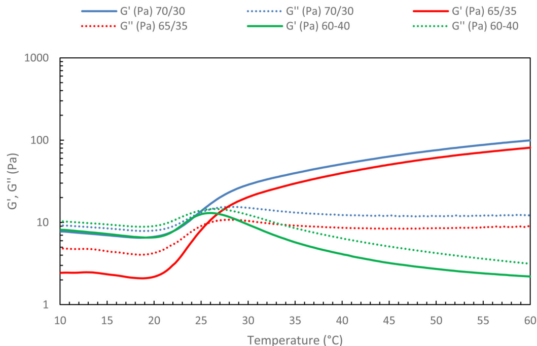
Fig. 11 Rheological ramp of different mixture between HA- g -P(iPrOx-co-BuOx-67/33)-0.10 and native HA ( 15 \text{ g L}^{-1} in NaCl 0.15 M; 0.5 \text{ }^\circ\text{C min}^{-1} , 0.1 Pa and 1 Hz).
