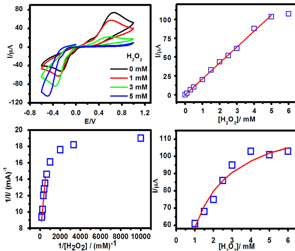
Fig. 4 (a) CV curves of PNP-OCDs@HRP in PBS with an increasing concentration of H_2O_2 in 3 mM HQ at a scan rate of 50 mV s -1 ranging from 1 to -0.6 V vs. Ag/AgCl and (b) cyclic voltammetric reduction current response in 3 mM HQ at a scan rate of 50 mV s -1 ranging from 1 to -0.6 V vs. Ag/AgCl of PNP-OCDs@HRP towards H_2O_2 addition. (c) Lineweaver-Burk plot for a current response of PNP-OCDs@HRP towards H_2O_2 addition, and (d) cyclic voltammetric reduction current response towards H_2O_2 addition with the fitted curve based on the Michaelis-Menten equation.
