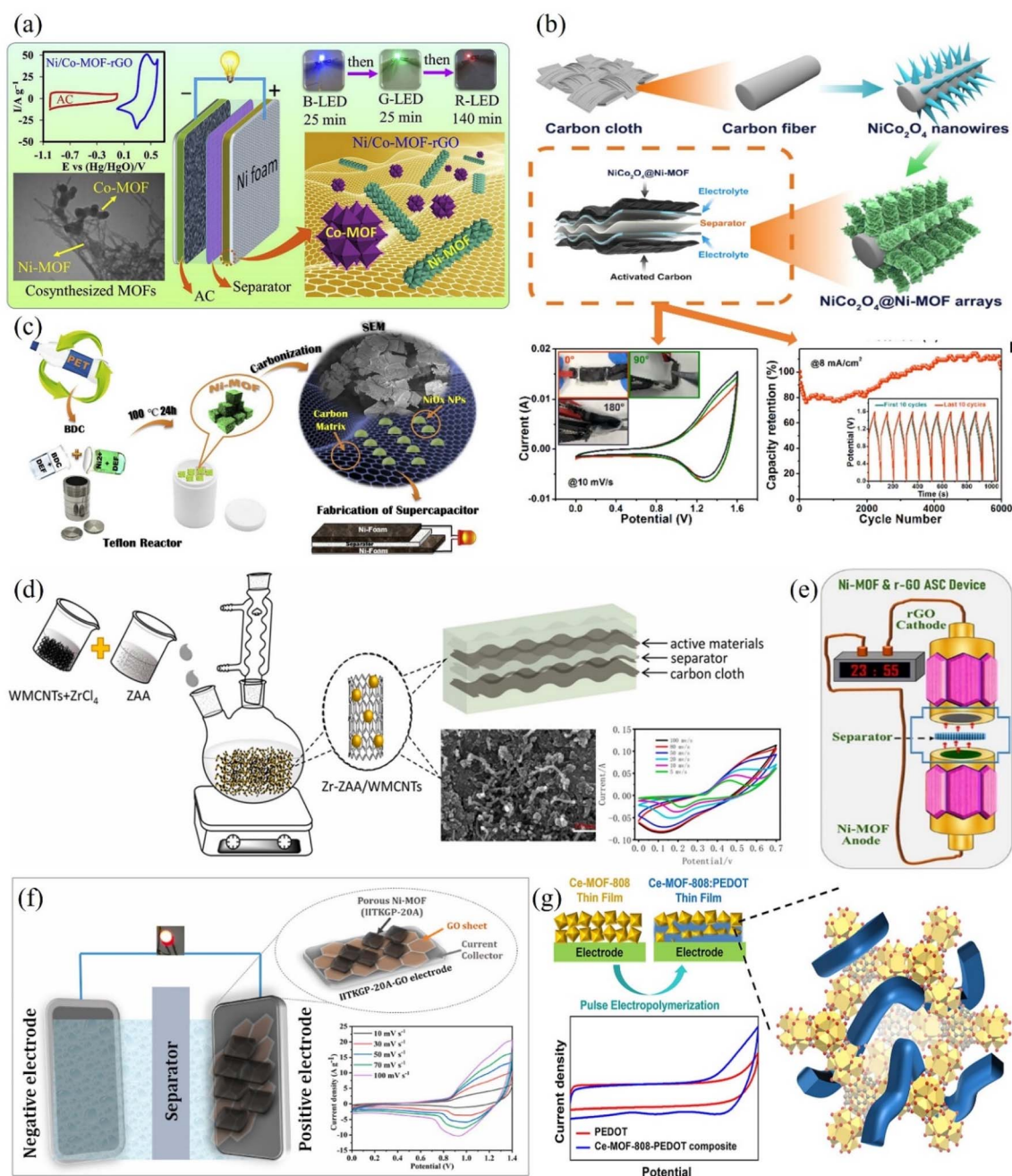
Fig. 6 (a) An asymmetric AC//Ni/Co-MOF-rGO device showing a capacitance of 860 \text{ F/g} at 1.0 \text{ A/g} in a 3E cell setup. Adopted from ref. 128 with permission. (b) A schematic depiction of the synthetic method employed to create core/shell hybrid arrays of \text{NiCo}_2\text{O}_4 @Ni-MOF on a carbon cloth substrate and the corresponding CV curves, and cycling stability tested at 8 \text{ mA/cm}^2 . Adopted from ref. 129 with permission. (c) Schematic diagram of the proposed method of synthesizing \text{NiO}_x @NPC nanocomposites using waste PET with enhanced electrical conductivity and stability and improved charge relocation operation for a better performance of supercapacitor devices. Adopted from ref. 113 with permission. (d) A novel electrode material, composed of MOFs (Zr-TAA, where TAA is trans -aconitic acid) and MWCNTs synthesized using a simple one-pot reflux method and applied to high-performance supercapacitors. Adopted from ref. 130 with permission. (e) A three-dimensional Ni-MOF used as an anode electrode in a two-electrode asymmetric supercapacitor device setup. Adopted from ref. 114 with permission. (f) Highly scalable and pH stable 2D Ni-MOF-based composites (IITKGP-20A-GO) for high-performance supercapacitors exhibiting a specific capacitance of \sim 840 \text{ F/g} at 2 \text{ A/g} current density. Adopted from ref. 131 with permission. (g) A cerium-based MOF@conducting polymer (PEDOT) nanocomposites for supercapacitors. Adopted from ref. 132 with permission.
