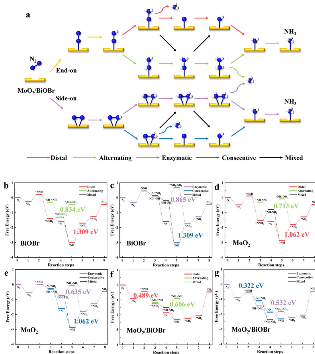
Fig. 8 (a) Schematic diagram of various reaction pathways for nitrogen reduction to synthesize ammonia; free energy diagrams for the five reaction paths on (b and c) BiOBr, (d and e) \text{MoO}_2 and (f and g) \text{MoO}_2/\text{BiOBr} . Note: the numbers in the diagrams are the values of the potential decision step (PDS).
