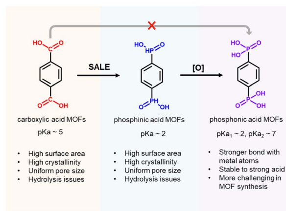
Scheme 1 Advantages of Zr–phosphinate/phosphonate MOFs.
