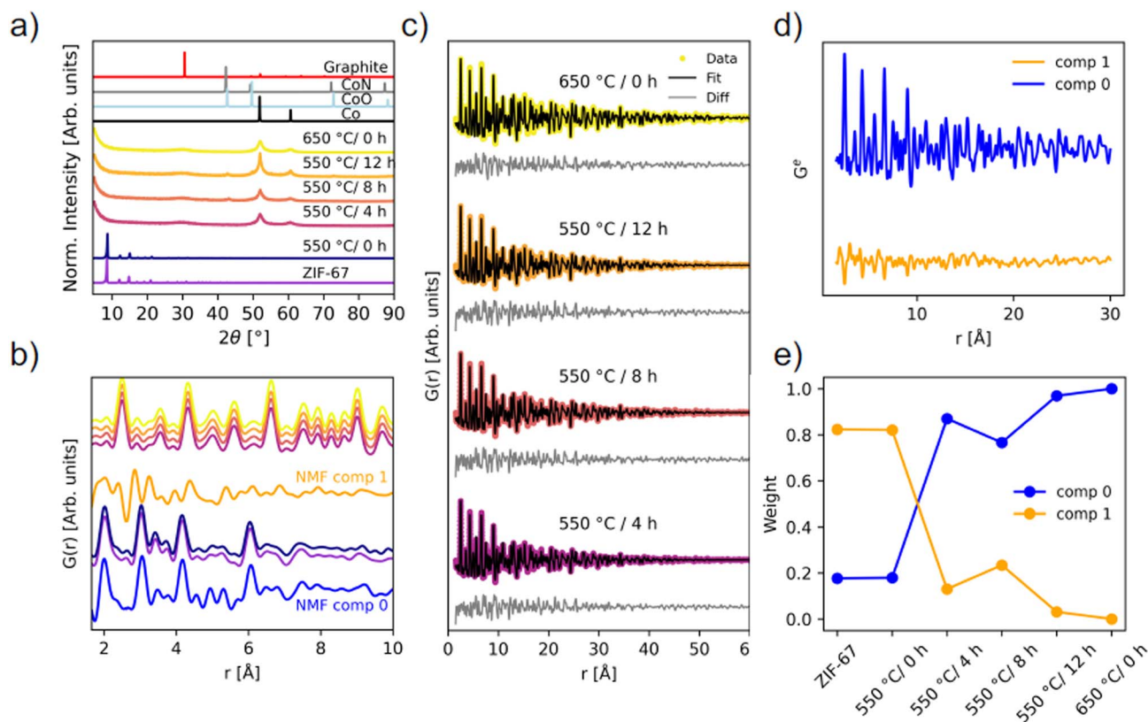
Fig. 6 Ex situ scattering experiments. (a) PXRD patterns ( \lambda = 1.79 Å) compared with calculated diffraction patterns of graphite (ICSD 31170 (ref. 49)), CoN (ICSD 79936 (ref. 45)), CoO (ICSD 9865 (ref. 50)), and Co metal (ICSD 76632 (ref. 44)). (b) PDFs of the local structure with identical color coding as in (a), compared with NMF components from the in situ experiment. (c) Two-phase PDF refinements of the four pyrolyzed samples that have converted into metallic Co. (d) NMF components, and (e) the weight of the NMF components used to recreate the experimental PDFs of each of the ex situ samples.
