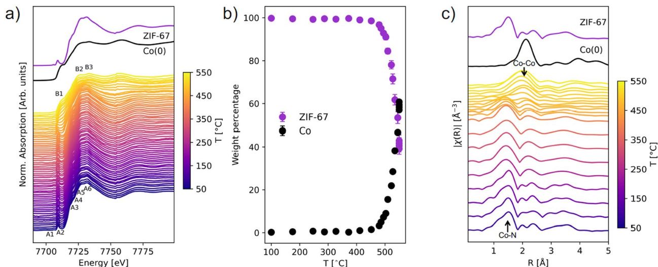
Fig. 2 (a) In situ XANES spectra of ZIF-67 during pyrolysis at 3 °C min −1 . The spectra are compared with that of an as-synthesized sample of ZIF-67 and a metallic Co(0) foil as reference spectra. Features in the ZIF-67 spectrum are annotated as A1–A6 and features of Co(0) as B1–B3. (b) Phase content evolution during ZIF-67 pyrolysis in weight percentage, based on LCA fitting. Two reference spectra were fitted to the data: ZIF-67 and metallic cobalt. (c) The Fourier transform magnitudes in R -space (not phase corrected) of the in situ EXAFS compared to the spectra of pristine ZIF-67 and metallic cobalt. From room temperature to 450 °C, every ten spectra have been merged, while above 450 °C every two spectra have been merged to capture the rapid changes.
