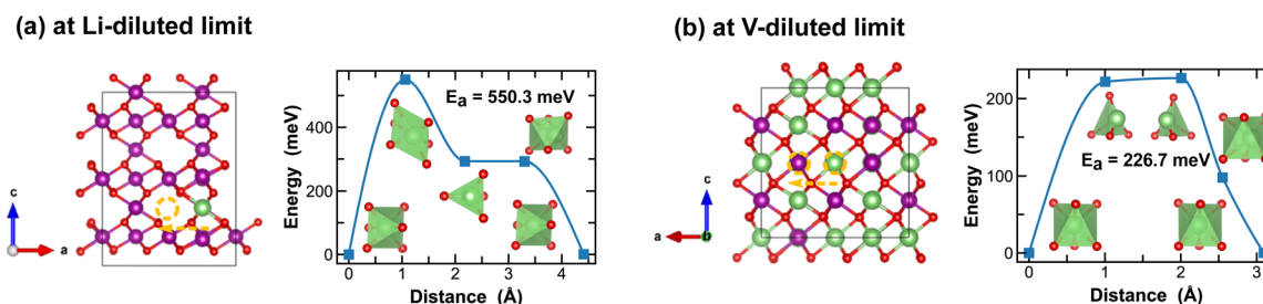
Fig. 10 Li-ion diffusion pathways identified at lithium- and vacancy diluted limits (in \epsilon - \text{MnO}_2 and \text{LiMnO}_2 , respectively), with the predicted energy barriers, E_a , in meV.
