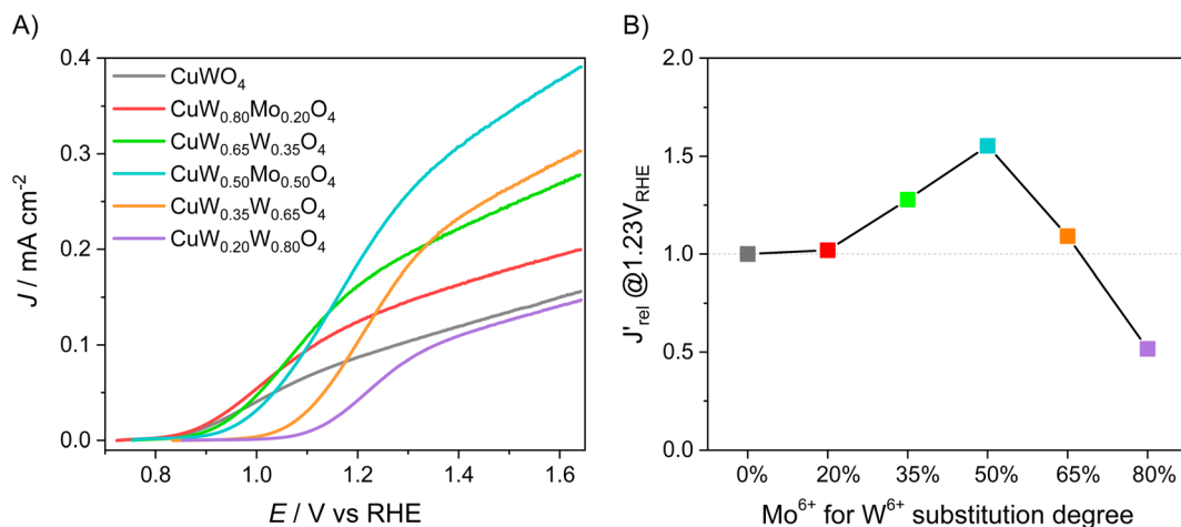
Fig. 2 (A) Linear sweep voltammetry (LSV) scans of CuW 1-x Mo x O 4 films with different Mo 6+ for W 6+ substitution degrees, under back-side irradiation. (B) Trend of the relative photocurrent efficiency J'_{rel} , defined in the main text, vs. the percent of Mo for W substitution degree.
