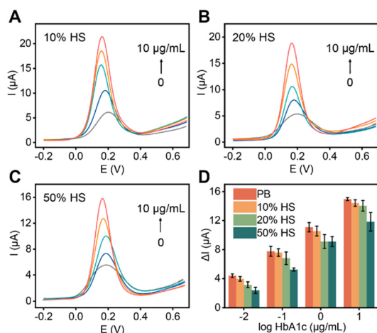
Fig. 5 SWV curves of this CRISPR-amplified aptasensor for the detection of different concentrations of HbA1c in (A) 10% human serum, (B) 20% human serum and (C) 50% human serum. (D) \Delta I of the aptasensor was tested in PB, 10%, 20% and 50% human serum for the detection of 0.01, 0.1, 1 and 10 \mu\text{g mL}^{-1} HbA1c.
