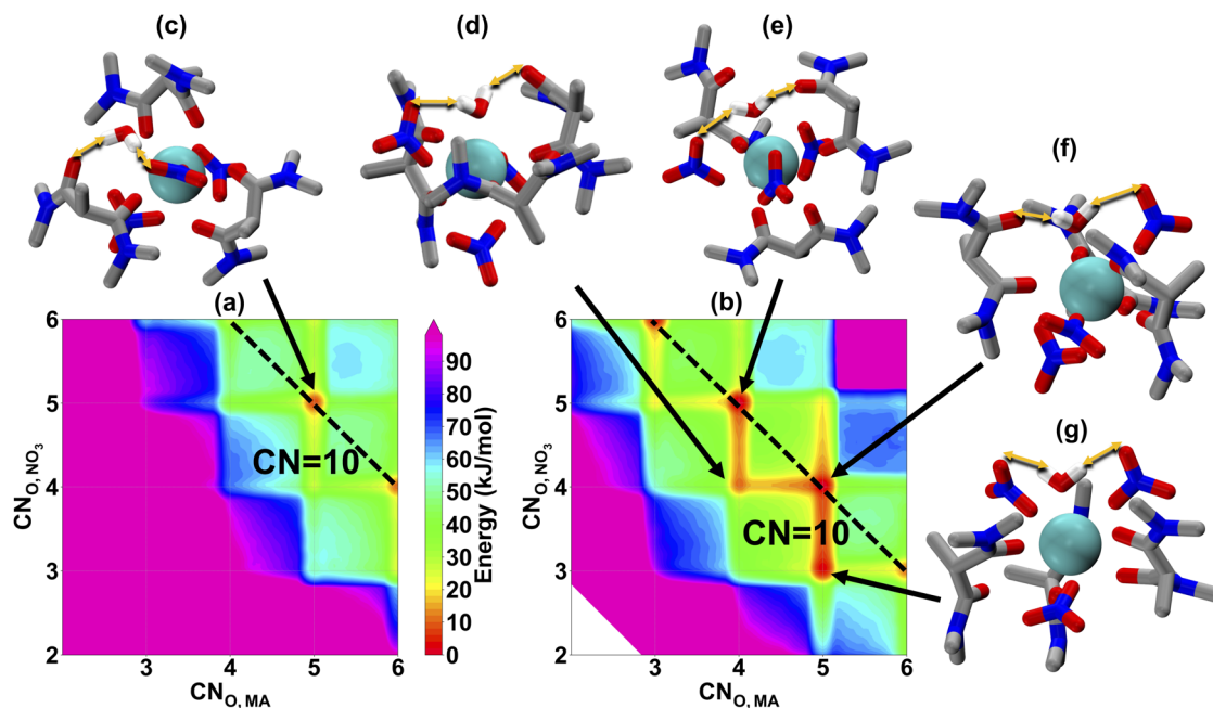
Fig. 2 \text{La(III)} solvation free energy landscapes in hexane from MD. x - and y -axis in (a) and (b) show the \text{CN}_{\text{O,MA}} and \text{CN}_{\text{O,NO}_3} respectively. (a) shows the solvation free energy landscape when water at the out-sphere ( \text{CN}_{\text{O,H}_2\text{O}} = 0 ), while (b) shows the same when water at the inner-sphere ( \text{CN}_{\text{O,H}_2\text{O}} = 1 ). A total coordination number of 10 is denoted by the dashed black line. (c)–(g) shows representative molecular events labeled by black arrows on the map. Hydrocarbon tails of MAs are replaced with the methyl group for simplicity. Yellow double arrows represent h-bond events.
