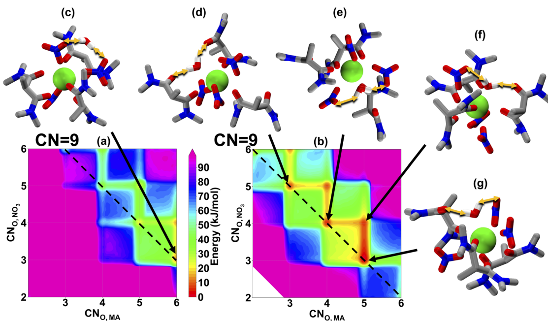
Fig. 3 \text{Eu(III)} solvation free energy landscapes in hexane from MD. x - and y -axis in (a) and (b) show the \text{CN}_{\text{O,MA}} and \text{CN}_{\text{O,NO}_3} respectively. (a) shows the solvation free energy landscape when water at the out-sphere ( \text{CN}_{\text{O,H}_2\text{O}} = 0 ), while (b) shows the same when water at the inner-sphere ( \text{CN}_{\text{O,H}_2\text{O}} = 1 ). A total coordination number of 9 is denoted by the dashed black line. (c)–(g) shows representative molecular events labeled by black arrows on the map. Hydrocarbon tails of MA are replaced with the methyl group for simplicity. Yellow double arrows represent h-bond events.
