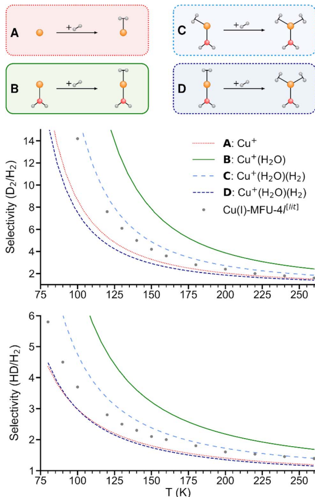
Fig. 5 Predicted selectivities for dihydrogen isotopologue adsorption at \text{Cu}^+ , \text{Cu}^+(\text{H}_2\text{O}) , and \text{Cu}^+(\text{H}_2\text{O})(\text{H}_2)_2 as a function of temperature. For the latter, two models are compared (see text). Literature data of Cu(I)-MFU-4l are shown for comparison. 4
