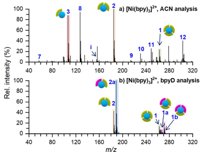
Fig. 2 Ex situ nano-DESI MS of the deposition spots of [Ni(bpy) 3 ] 2+ analyzed with (a) ACN and (b) 3 μM bpyD in ACN as the nano-DESI solvent. Ion assignments are listed in Table 1. The pictograms symbolize the number of ligands coordinated to Ni. Green and pink symbols represent bpy and bpyD, respectively. Peaks originating from the solvent are not marked in the spectra for simplicity.
