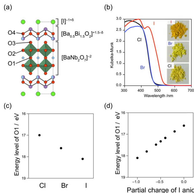
Fig. 13 (a) Crystal structure of Bi_3Ba_2Nb_2O_{11} , showing the effective charges of I and Bi(2). (b) Diffuse reflectance spectra and sample color of Bi_3Ba_2Nb_2O_{11}X ( X = Cl, Br, I ). (c) Ionic energy levels of O^{2-} at the O1 site in Ba_2Bi_3Nb_2O_{11} , which contributes to the VBM obtained by using the Madelung potential calculated using formal charges. (d) Ionic energy levels at the O1 site, calculated under different assumptions of the effective charge of the iodide anion considering its softness. (b–d) Adapted with permission from ref. 109 Copyright 2021, American Chemical Society.
