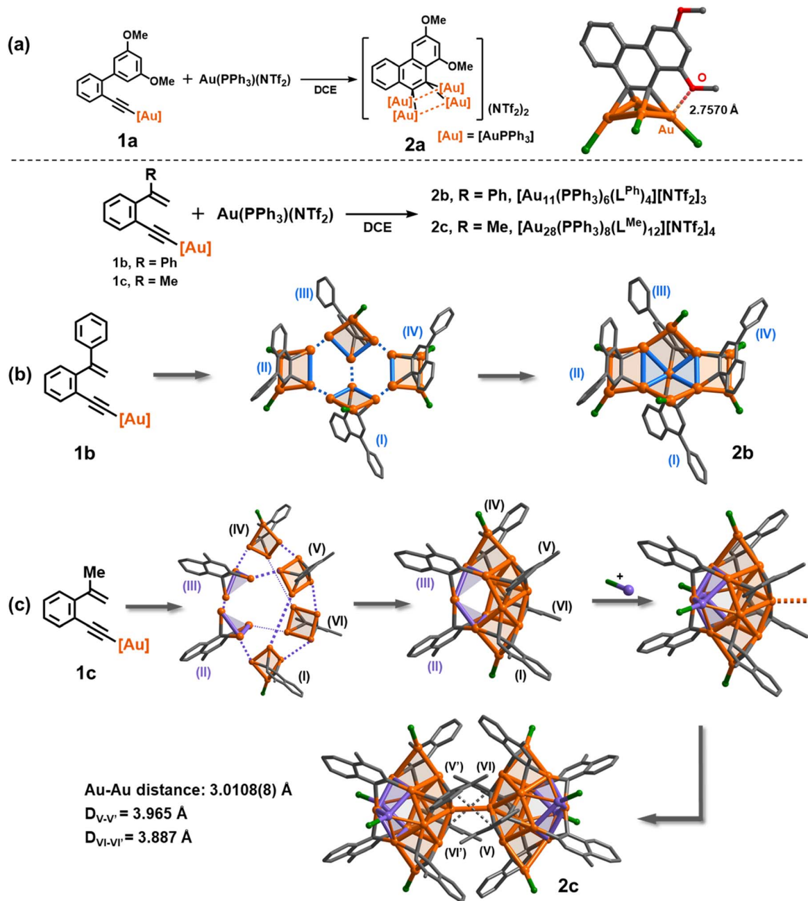
Fig. 1 Synthesis, crystal structures and assembled patterns of (a) discrete vicinal dicarbanion-bonded tetragold cluster 2a , (b) net-like cluster 2b , and (c) dumbbell-like cluster 2c . Hydrogen atoms, phenyl groups of \text{PPh}_3 ligands and peripheral \text{NTf}_2^- counter anions are omitted for clarity. Color coding: Au, orange and purple; C, gray; O, red; P, green.
