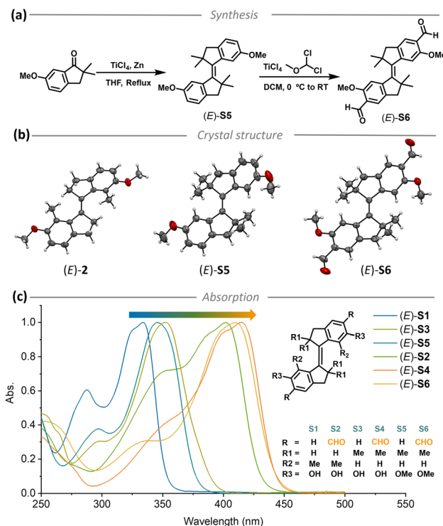
Fig. 2 (a) The synthesis of stiff-stilbene derivatives ( E - S5 and ( E - S6 by McMurry coupling and Rieche formylation, (b) crystal structures of ( E )- 2 , ( E - S5 , and ( E - S6 , (c) molecular structures of ( E - S1 to ( E - S6 and the normalized steady-state absorption spectra of ( E - S1 to ( E - S6 (( E - S1 in DMSO and others in CH 2 Cl 2 , 298 K).
