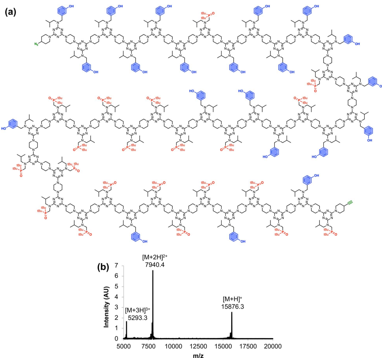
Fig. 6 (a) Chemical structure and (b) MALDI-TOF mass spectrum of the 42-mer REMO, zDDDDDDADDDDDADDADADAAAAADAAAA-DAAADAADy. Calculated masses: 15876.2 [M+H]^+ , 7940.1 [M+2H]^{2+} , 5293.4 [M+3H]^{3+} .
