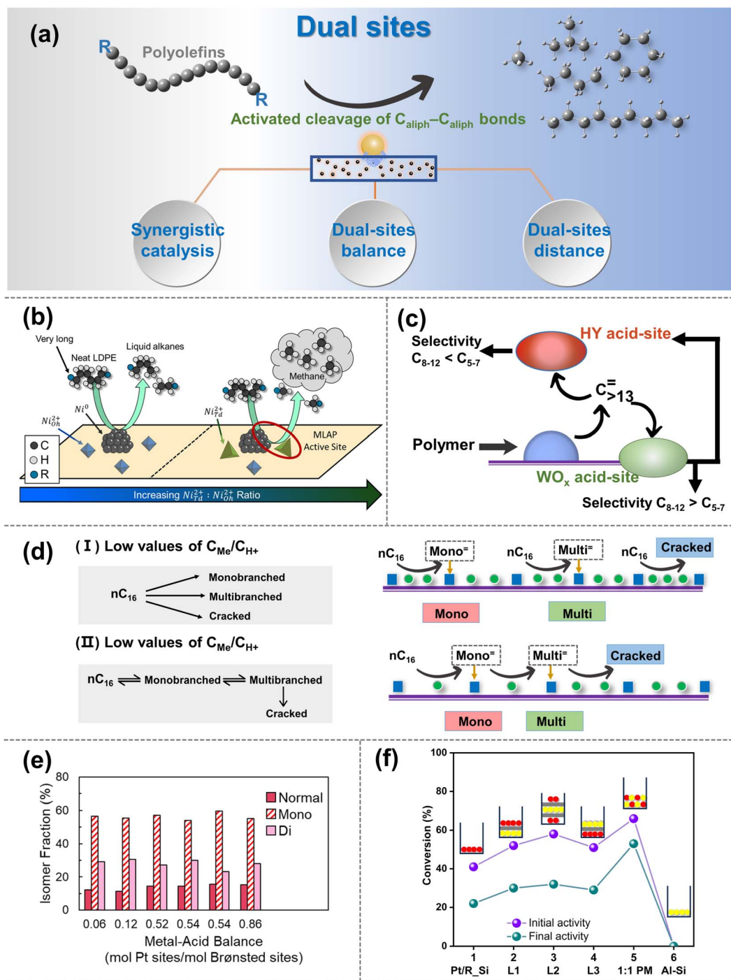
Fig. 5 (a) Schematic diagrams of the upgradation of polyolefins when the C_{\text{aliph}}-C_{\text{aliph}} activation occurs over the dual sites. (b) Schematic picture of the proposed mode by which \text{Ni}_{\text{Td}}^{2+} promotes methane production, selectivity comparisons are made at 25–45% LDPE deconstruction. Reproduced with permission from ref. 111. Copyright 2023 American Chemical Society. (c) Depiction of main intermediates diffusing over the Pt/ \text{WO}_3/\text{ZrO}_2 + HY(30) catalyst. Reproduced with permission from ref. 104. Copyright 2021 Science. (d) n -Hexadecane hydroisomerization mechanisms over the Me/S31 catalysts at: (I) low values of C_{\text{Me}}/C_{\text{H}^+} ; and (II) high values of C_{\text{Me}}/C_{\text{H}^+} . Reproduced with permission from ref. 117. Copyright 2018 Royal Society of Chemistry. (e) Fraction of normal, monobranched, and dibranched isomers in extractable LDPE hydrocracking over catalysts with different metal–acid balances (MABs). Data collected from ref. 102 and copyright 2021 Elsevier. (f) Conversion obtained for different two-component catalysts based on Pt/R Si and SIRAL80 (Al–Si). Reproduced with permission from ref. 119 and copyright 2016 Elsevier.
