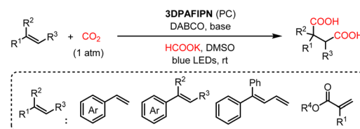
Scheme 1 The development of dicarboxylation of alkenes with formate and CO 2 .
