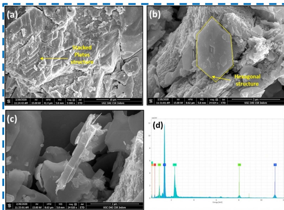
Fig. 9 (a–c) FESEM images (d) EDS of the synthesized \text{MoSe}_2 powder. This figure has been reproduced from ref. 66 with permission from Elsevier, Copyright 2020.
