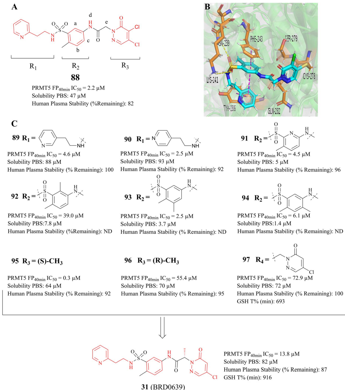
Fig. 14 (A) Lead compound 88 . (B) The cocrystal structure of compound 88 bound to the PRMT5 complex (PDB: 7M05). 31 (C) Further SAR exploration of 88 results in a PBM-competitive inhibitor 31 (BRD0639). The FP is a competition fluorescence polarization assay.
