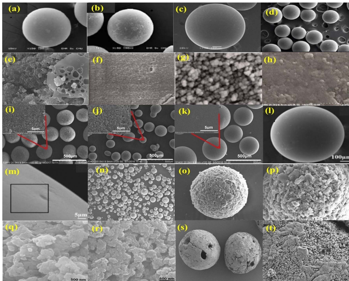
Fig. 5 SEM images of anion exchange resins (a) Dowex, 70 (b) FO-Dowex, 70 (c) De-Acidite FF-IP {reproduced from ref. 71 with permission from Elsevier (License number-5531250299948)}. (d) nZVI-402-Cl {reprinted (adapted) with permission from ref. 72 Copyright © 2022 American Chemical Society}. (e) PVC-based anion exchange resin {reproduced from ref. 73 with permission from Elsevier (License number-5531290655343)}. (f) polymeric anion exchanger {reproduced from ref. 74 with permission from Elsevier (License number-5531291287322)}, (g) polymeric anion exchanger decorated with magnetite nanoparticles {reproduced from ref. 74 with permission from Elsevier (License number-5531291287322)}, (h) NDP-2 resin {reproduced from ref. 75 with permission from Elsevier (License number-5531260219427)}, (i) L-20 resin {reproduced from ref. 76 with permission from Elsevier (License number-5533211402968)}, (j) ML-20 resin {reproduced from ref. 76 with permission from Elsevier (License number-5533211402968)}, (k) MIEX resin {reproduced from ref. 76 with permission from Elsevier (License number-5533211402968)}, (l) D201 resin {reprinted (adapted) with permission from ref. 77 Copyright © 2020 American Chemical Society}, (m) D201 resin after NO 3 - adsorption {reprinted (adapted) with permission from ref. 77 Copyright © 2020 American Chemical Society}, (n–p) MAER resin {reproduced from ref. 56 with permission from Elsevier (License number-5530880464787)}, (q and r) the Purolite A520E resin, magnetic resin {reproduced from ref. 78 with permission from Elsevier (License number-5794900244372)}, (s and t) MGE resin {reproduced from ref. 79 with permission from Elsevier (License number- 5794890063873)}.
