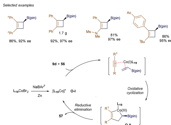
Scheme 21 Co(I)-catalyzed [2 + 2] cycloaddition.
