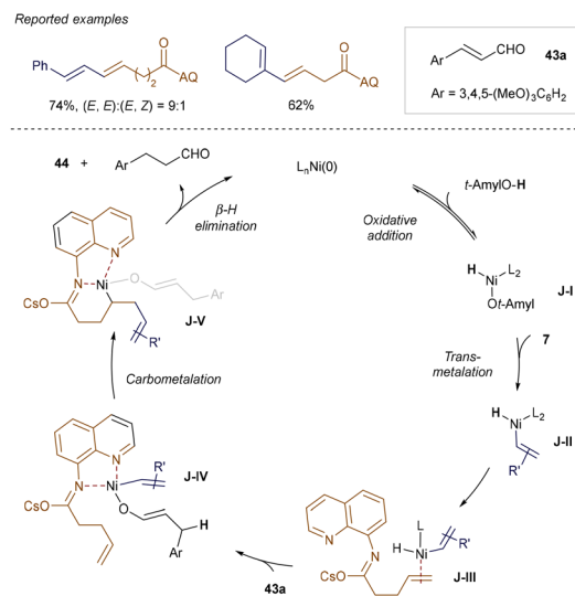
Scheme 14 Ni-catalyzed oxidative Heck reaction.
