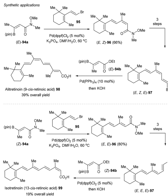
Scheme 37 Synthetic applications.
