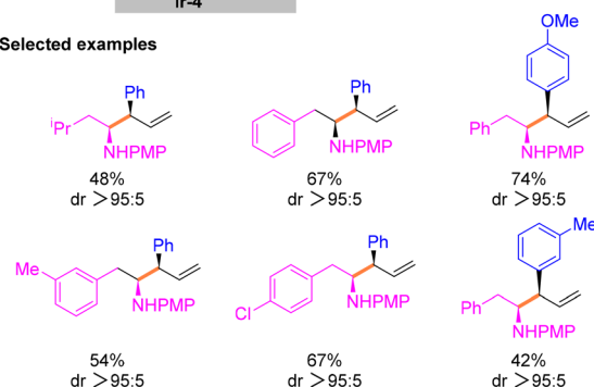
Scheme 10 Synthesis of homoallyl amines by a cross-coupling reaction.
