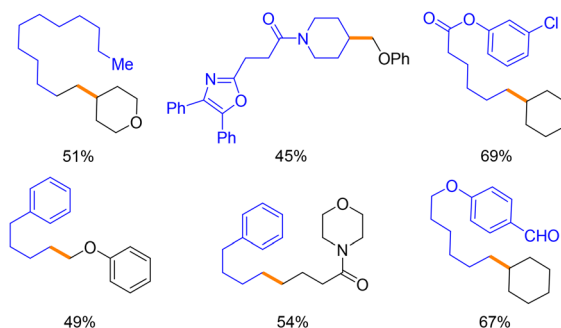
Scheme 9 Csp 3 –Csp 3 cross-coupling reaction of dihydroquinazolinones with bromoalkanes.
