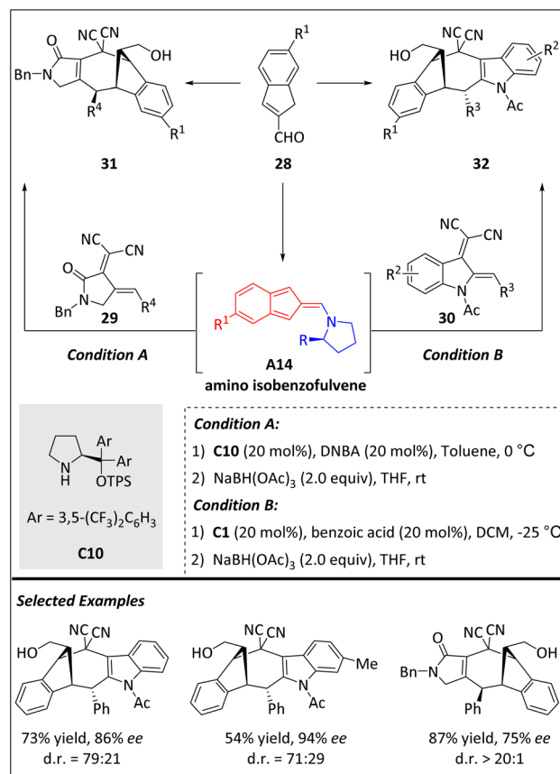
Scheme 10 Asymmetric intermolecular [8 + 4] cycloadditions via the amino isobenzofulvene intermediate.
