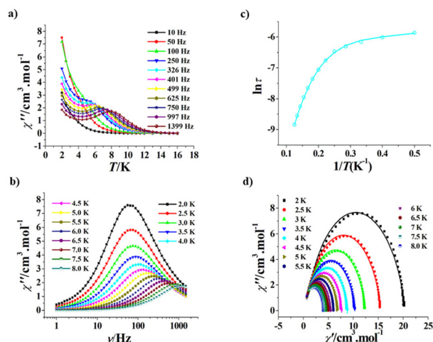
Fig. 6 Plots of \chi'' versus T for D-1 ( H_{dc} = 0 Oe) (a). Frequency dependence of \chi'' for D-1 at a zero dc field (b). Plot of \ln(\tau) versus 1/T for D-1 ( H_{dc} = 0 Oe); the solid line represents the best fitting with quantum tunnelling plus Orbach plus Raman (c). Cole–Cole plots measured from 2.0 to 8.0 K for D-1 ( H_{dc} = 0 Oe); the solid lines represent the best fitting with the generalized Debye model (d).
