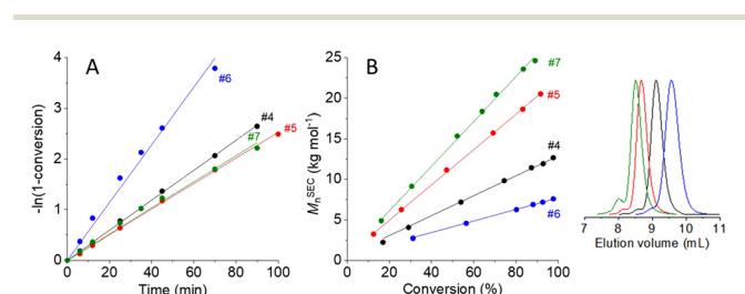
Fig. 1 (A) Pseudo first-order time-conversion plots for the sec -butyllithium initiated anionic polymerizations of \beta -myrcene in DL-limonene at room temperature (Table 1, #4–7). (B) Evolution of the number-average molar mass, M_n^{SEC} , as a function of monomer conversion and SEC traces of the final polymyrcene samples #4–7.
