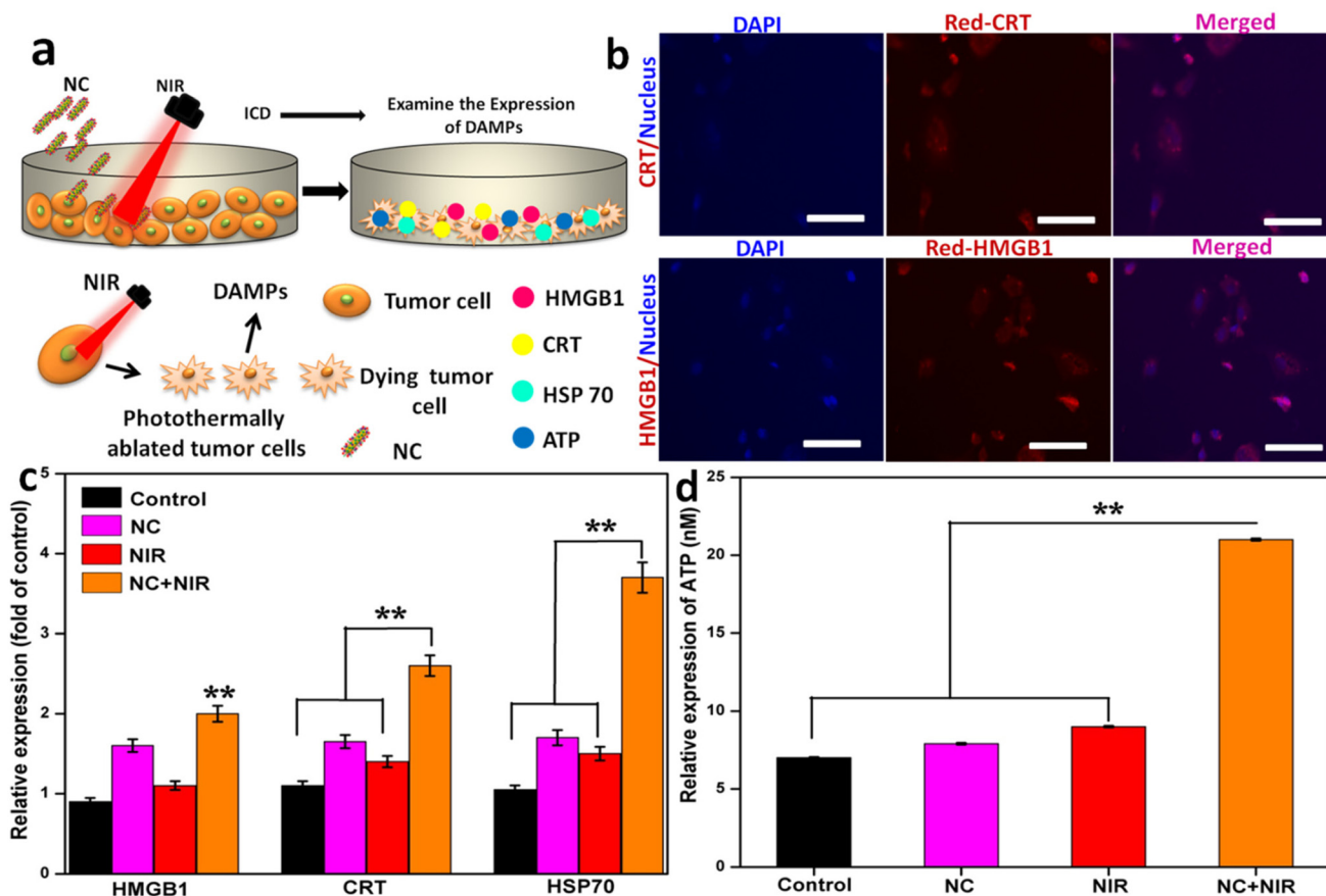
Fig. 7 (a) Schematic illustration of the experiment. (b) Immunofluorescence analysis of HMGB1, and CRT expression after the above-indicated treatment. Scale bar: 20 μm. (c) Quantitative analysis of HMGB1, CRT, and HSP70. (d) ATP expression. (Mean \pm S.D., n = 3 . Student's t -test, *P < 0.05 ; **P < 0.01 vs. control).
