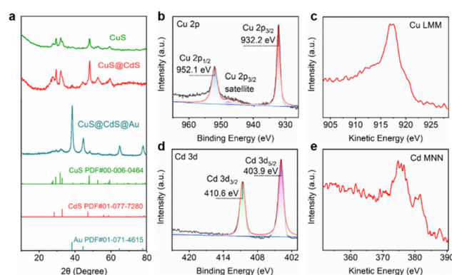
Fig. 2 (a) XRD patterns of CuS, \text{CuS@CdS} , and \text{CuS@CdS@Au} NSs and their corresponding standard PDF cards. XPS spectra of (b) Cu 2p, (c) Cu LMM, (d) Cd 3d, and (e) Cd MNN in \text{CuS@CdS@Au} NSs.
