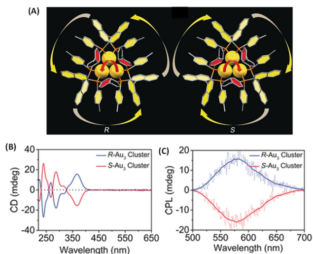
Fig. 7 (A) The overall structures of R/S - Au_3 . Color codes: Au, yellow; P, orange; C, gray. (B) CD spectra of Au_3(R) -Tol-BINAP 3 Cl and Au_3(S) -Tol-BINAP 3 Cl clusters in DCM. (C) CPL spectra of R - Au_3 and S - Au_3 assemblies in 70% n -hexane. (Reproduced from ref. 45 with permission from John Wiley and Sons, Copyright 2017).
