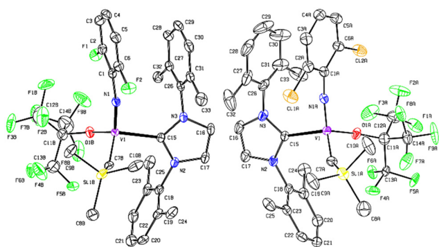
Fig. 3 ORTEP drawings for [V(N-2,6-X 2 C 6 H 3 )(CHSiMe 3 )(OC(CF 3 ) 3 )(NHC)] [X = F ( 3 , left), Cl ( 4 , right)]. Hydrogen atoms were omitted for clarity and thermal ellipsoids are drawn at 30% probability level. Additional data including crystal data and collection parameters for structural analysis are shown in ESI.†
