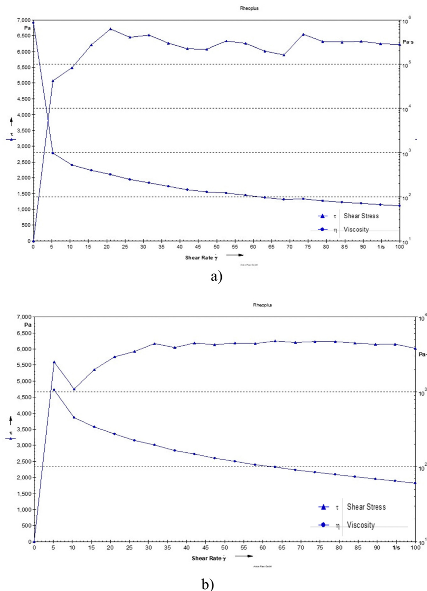
Fig. 5 Shear stress of (a) the blank hydrogel and (b) the drug-loaded hydrogel as a function of shear rate.
