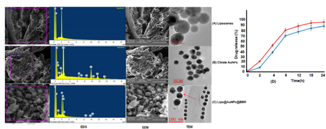
Fig. 4 TEM and SEM images and EDS spectra of liposome (A), citrate AuNPs (B) and Lipo@AuNPs@BBR (C) nanoparticles. (D) The in vitro drug release of citrate AuNPs and BBR from the Lipo@AuNPs@BBR complex was measured via dialysis in PBS (pH = 7.4) at room temperature for 24 h. As can be seen, citrate AuNPs were released with more speed than BBR from the Lipo@AuNPs@BBR complex.
