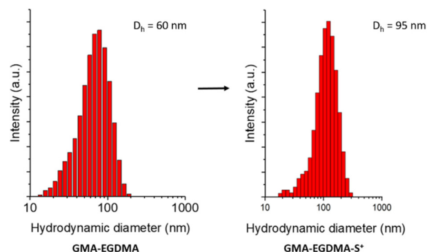
Fig. 4 The hydrodynamic diameters of GMA-EGDMA-S + (in 5 mM KCl) and GMA-EGDMA (in DCM) were measured by means of DLS indicating a semi bimodal size distribution. This increase in size is likely the result of same charges repelling each other as well as a difference in solvents.
