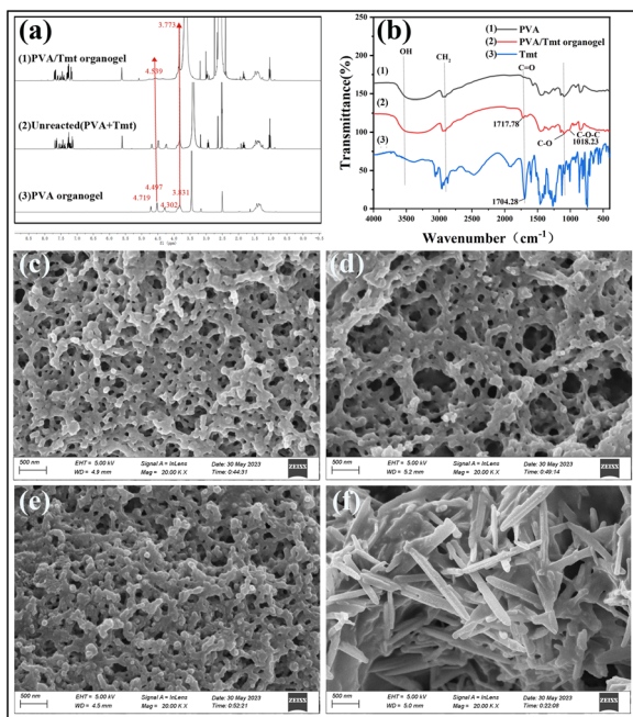
Fig. 2 (a) 1 H NMR and (b) FT-IR spectra of the different samples. Field-emission scanning electron microscopy (SEM) images of (c) PVA, (d) PVA/Tmt, (e) PVA/Tmt/RhB and (f) PVA/Tmt/AYG organogel samples.
