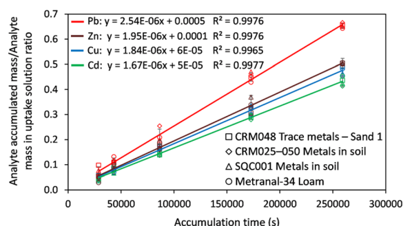
Fig. 2 Uptake kinetics of target elements by Chelex-100 DGT for the uptake solution prepared from four CRMs. Conditions: volume of the uptake solution: 100 mL prepared by 10-fold dilution of the digested CRMs; pH: 4.0 \pm 0.1 ; temperature: 21 \pm 1^\circ\text{C} ; elution in 1 mL solution of 1\text{ mol L}^{-1}\text{ HNO}_3 . Error bars correspond to the standard deviation obtained for the four CRMs.
