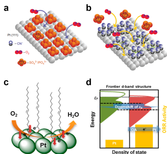
Fig. 10 (a) On Pt(111) covered by phosphoric/sulfuric acid anions, \text{O}_2 can access the surface's atoms only through a small number of holes in the adsorbate anion adlayer; (b) the number of holes required for \text{O}_2 adsorption is significantly increased on the Pt(111)– \text{CN}_{\text{ad}} surface because adsorption of phosphoric/sulfuric acid anions is suppressed by the CN adlayer so that the total \text{CN}_{\text{ad}}/\text{OH}_{\text{ad}} coverage is lower than the coverage by sulfuric or phosphoric acid anions. Reprinted with permission from ref. 55 Copyright 2010, Springer Nature. (c and d) Schematic presentation of tailoring the d-band structure by surface-capping organic molecules. Reprinted with permission from ref. 56. Copyright 2013, American Chemical Society.
