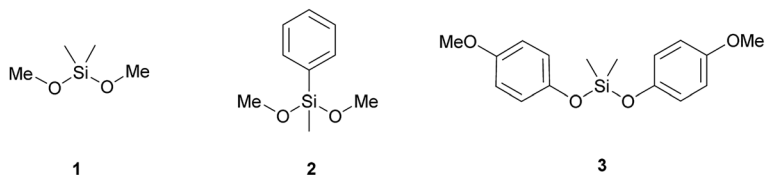
Fig. 2 Structures of the precursor molecules used as enzyme substrates in this study.
