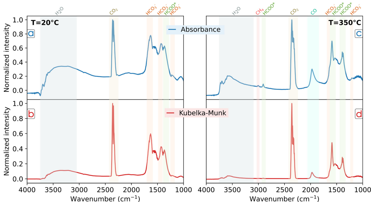
Fig. 4 Comparison of absorbance vs. Kubelka-Munk spectra taken during NTP \text{CO}_2 hydrogenation over \text{Co}/\text{Al}_2\text{O}_3 . The DRIFTS cell temperature was controlled at 20 °C (a) and (b), and 350 °C (c) and (d). Data were collected in a custom modified DBD DRIFTS cell at 4000 V and 10 kHz with 36 sccm of Ar, 1 sccm of \text{CO}_2 , and 3 sccm of \text{H}_2 .
