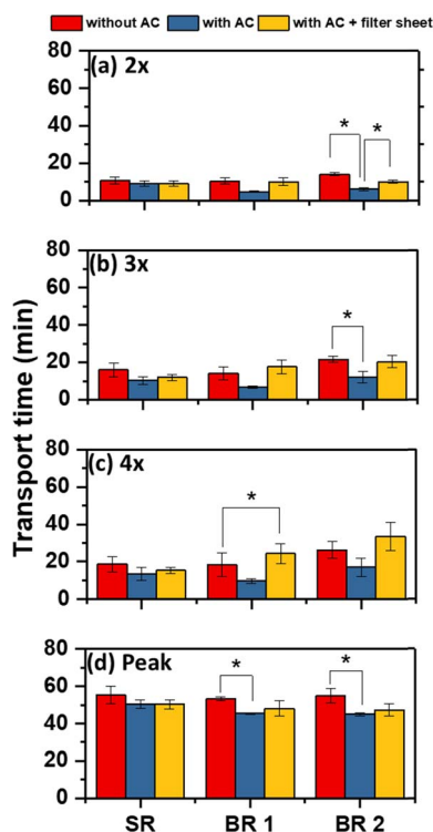
Fig. 3 Time for the concentrations in the study room (SR), bedroom 1 (BR 1), and bedroom 2 (BR 2) to reach (a) 2\times , (b) 3\times , (c) 4\times , and (d) peak relative to the background concentration under three scenarios: without AC, with AC on, and with AC on + filter sheet, * with bracket shows the compared categories and presence of significance difference.
