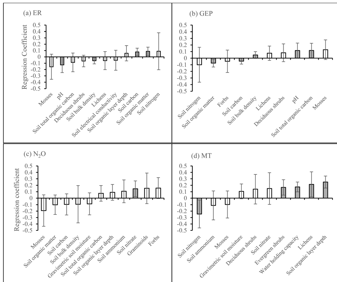
Fig. 6 Regression coefficients from PLS regression models on (a) ER, (b) GEP, (c) \text{N}_2\text{O} , and (d) MT during the first growing season. Error bars show \pm 2 standard deviations of the regression coefficients. Significant variables are marked with grey bars. The shown models for \text{N}_2\text{O} and MTs are significant (CV-ANOVA) at P < 0.05 .
