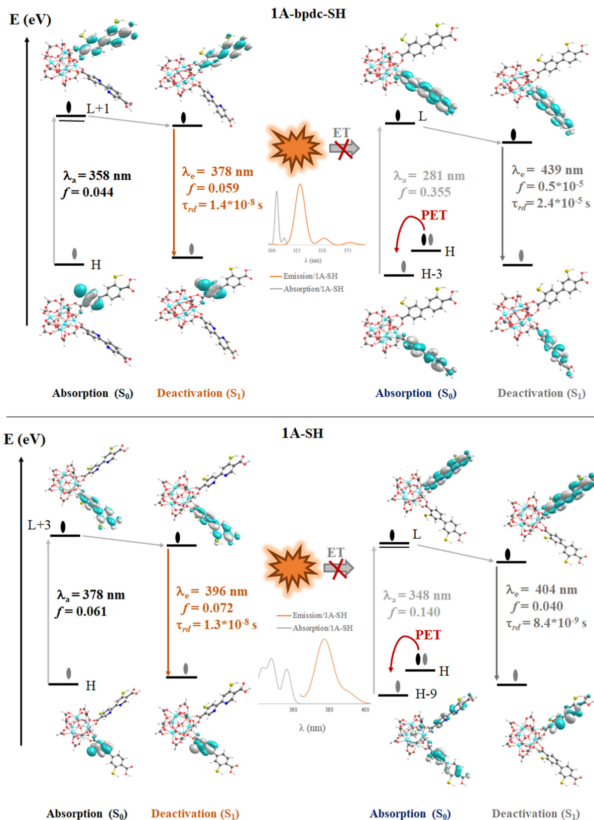
Fig. 7 Schematic representation of the photophysical mechanism based on FMOs analysis on the S_0 (absorption) and S_1 states to 1A-bpdc-SH and 1A-SH system. Where, \lambda_a and \lambda_e are the computed wavelength of absorption (gray) and deactivation (orange and dark gray), respectively; f is the oscillator strength; \tau_{rad} is the radiative transition lifetime and ET is energy transfer. The spectral overlap (emission bpdc/absorption at bpdc) is represented. Isosurface contour values are set as 0.03 with TDDFT/Def2-TZPP/B3LYP theory level.
