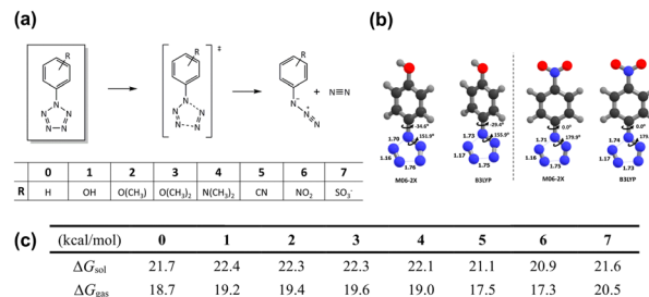
Fig. 1 (a) Schematic view for the decomposition of arylpentazoles with substituents 0–7; (b) selected geometries of transition state structures; (c) reaction barriers of decomposition of para -substituted arylpentazoles 0–7. Reproduced with permission from ref. 72. Copyright 2019, The Royal Society of Chemistry.
