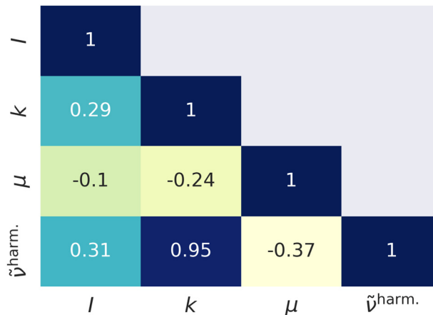
Fig. 2 Linear correlation coefficients of the descriptors. I – intensity of the harmonic vibration.
