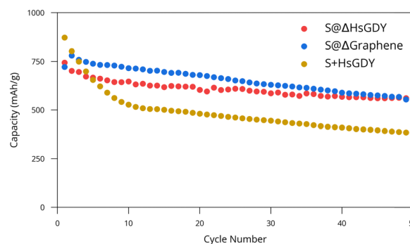
Fig. 4 Cycling performance of S@HsGDY, S@Δgraphene, and S+HsGDY. Best results are shown for each cathode material while triplicates are shown in Fig. S12 (ESI†). Capacity is in terms of mass of sulfur.
