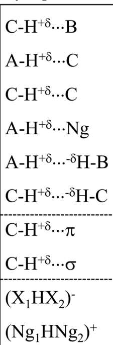
Scheme 2 Examples of the specific types of hydrogen bonds.
