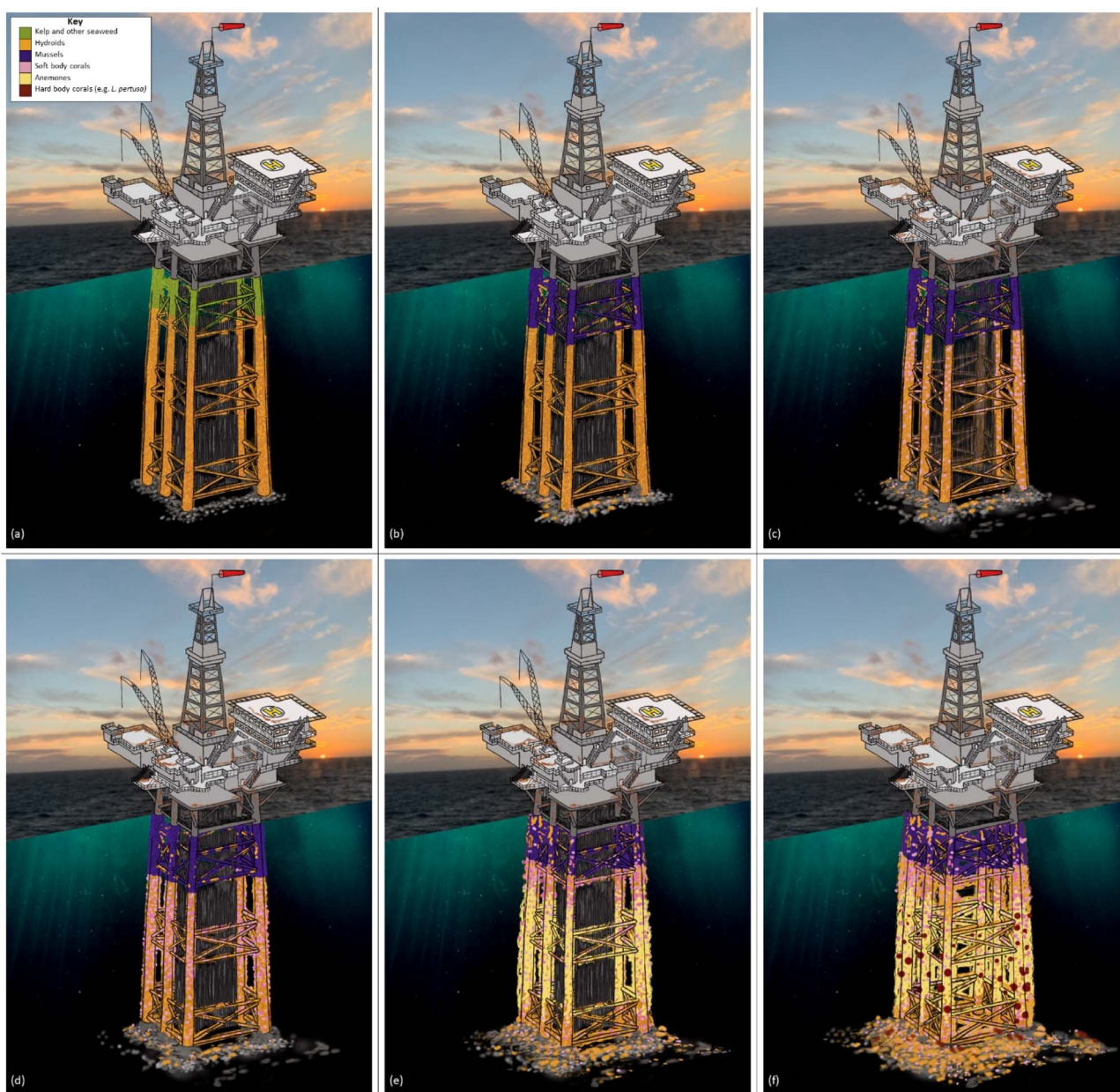
Fig. 5 Evolution of biomass adhered to OGI MMS. (a) 3 months after installation, (b) represents 5–10 years since installation, (c) 10–20 years after installation, (d) 20–30 years after installation, (e) 30–40 years after installation and (f) 50 years after installation. Diagrams (a–e) would be during the operational stage of producing HCs (hot phase) and (f) would be around the time of cold decommissioning, the well will be plugged and abandoned and no more HCs should be present. Data from ref. 8 and 18.
