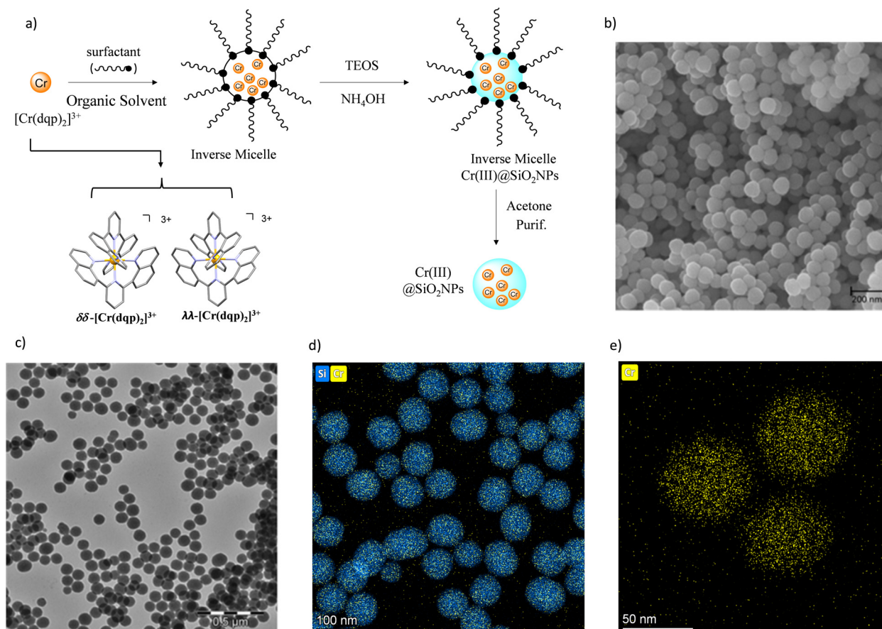
Fig. 3 (a) Schematic synthetic approach for preparing the silica nanoparticles (b) SEM image of the prepared rac -Cr@SiO 2 NPs nanoparticles (c) TEM image of the prepared λλ-Cr@SiO 2 NPs; (d) and (e) HAADF-STEM compositional mapping image of λλ-Cr@SiO 2 NPs.
